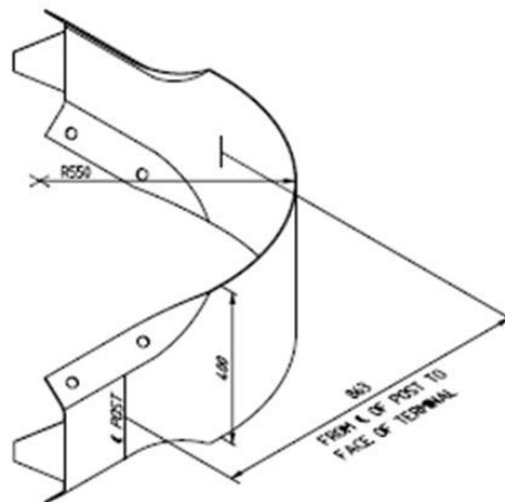
RIGHT ANGLE TERMINAL Part No. C1068G
