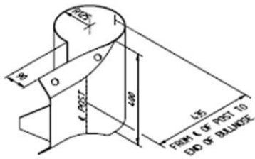
SHORT BULLNOSE Part No. C1064G
