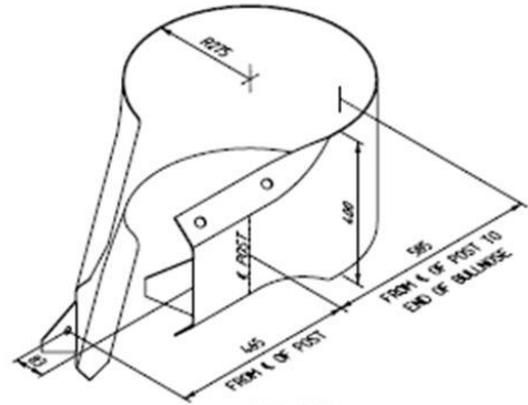
BULLNOSE Part No. C1060G
