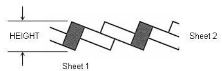
LAYING EXPANDED METAL SHEETS
