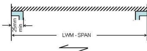
MINIMUM SUPPORT DIMENSION
